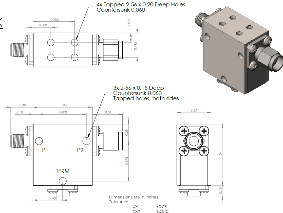
D3I3587YMG-77K-2 Dimensions
