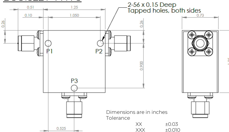
D3C1522Y-77K-3
