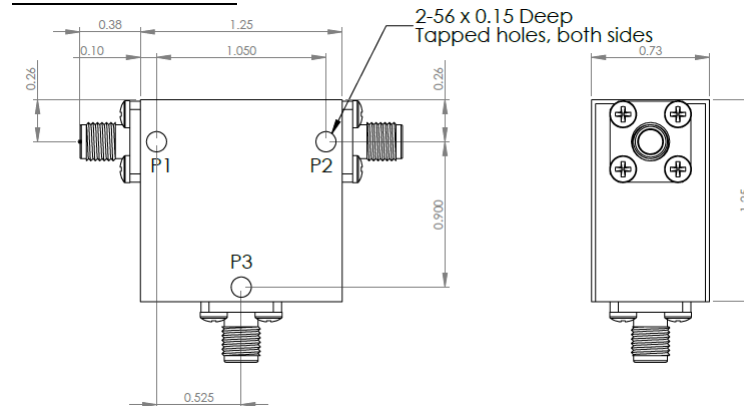
D3C1522Y-77K-3
