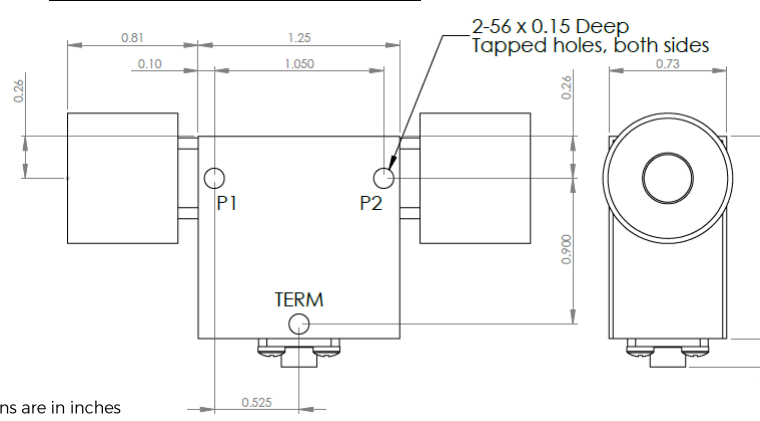
D3I2327N-3 Dimensions
