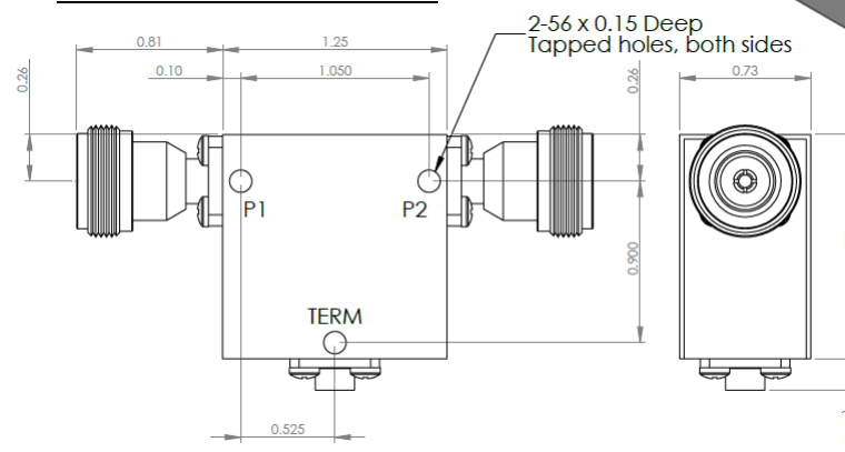
D3I2327N-3 Dimensions
